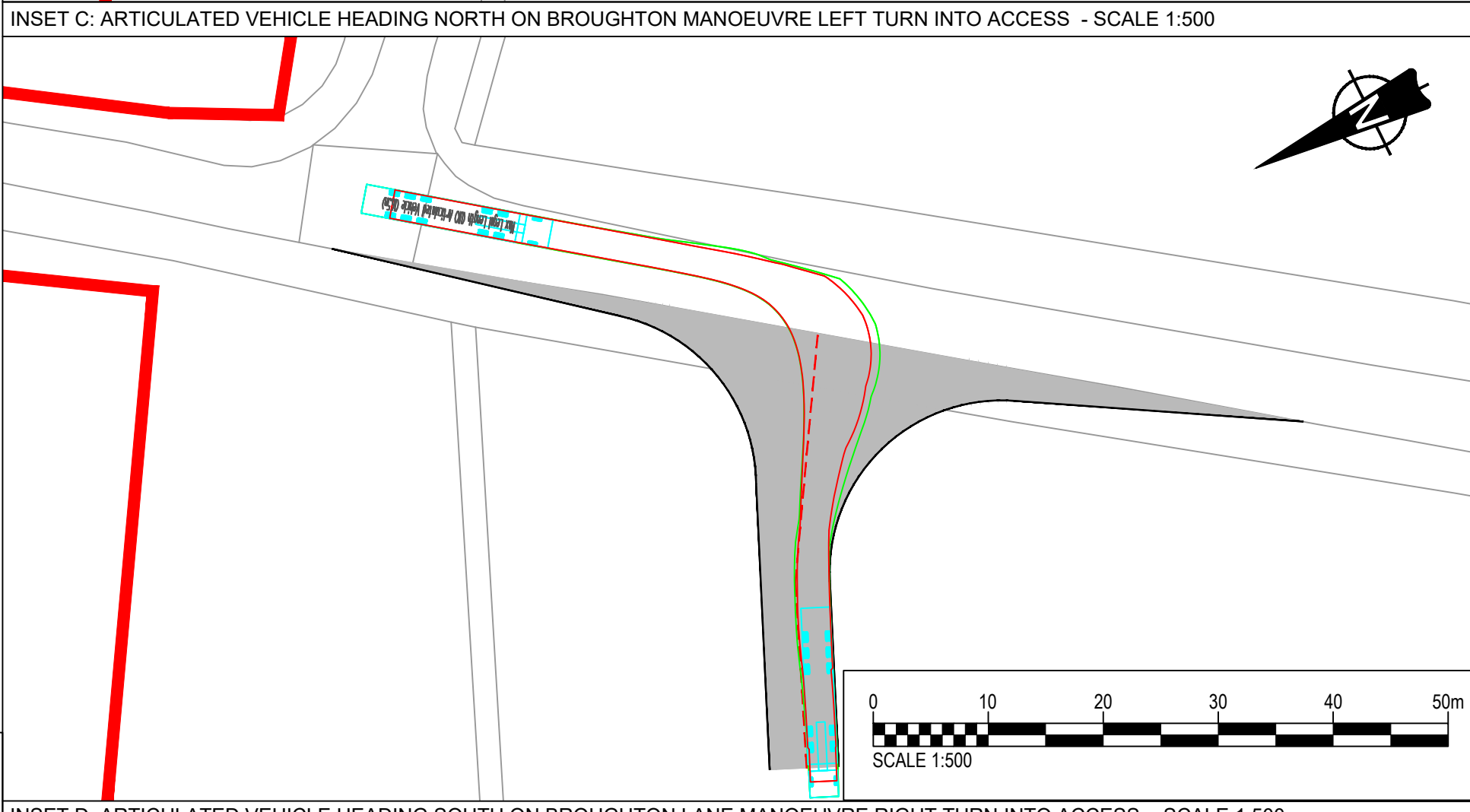
INSET D: ARTICULATED VEHICLE HEADING SOUTH ON BROUGHTON LANE MANOEUVRE RIGHT TURN INTO ACCESS - SCALE 1:500
