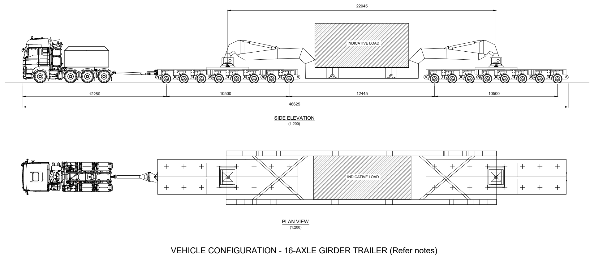
VEHICLE CONFIGURATION - 16-AXLE GIRDER TRAILER (Refer notes)
