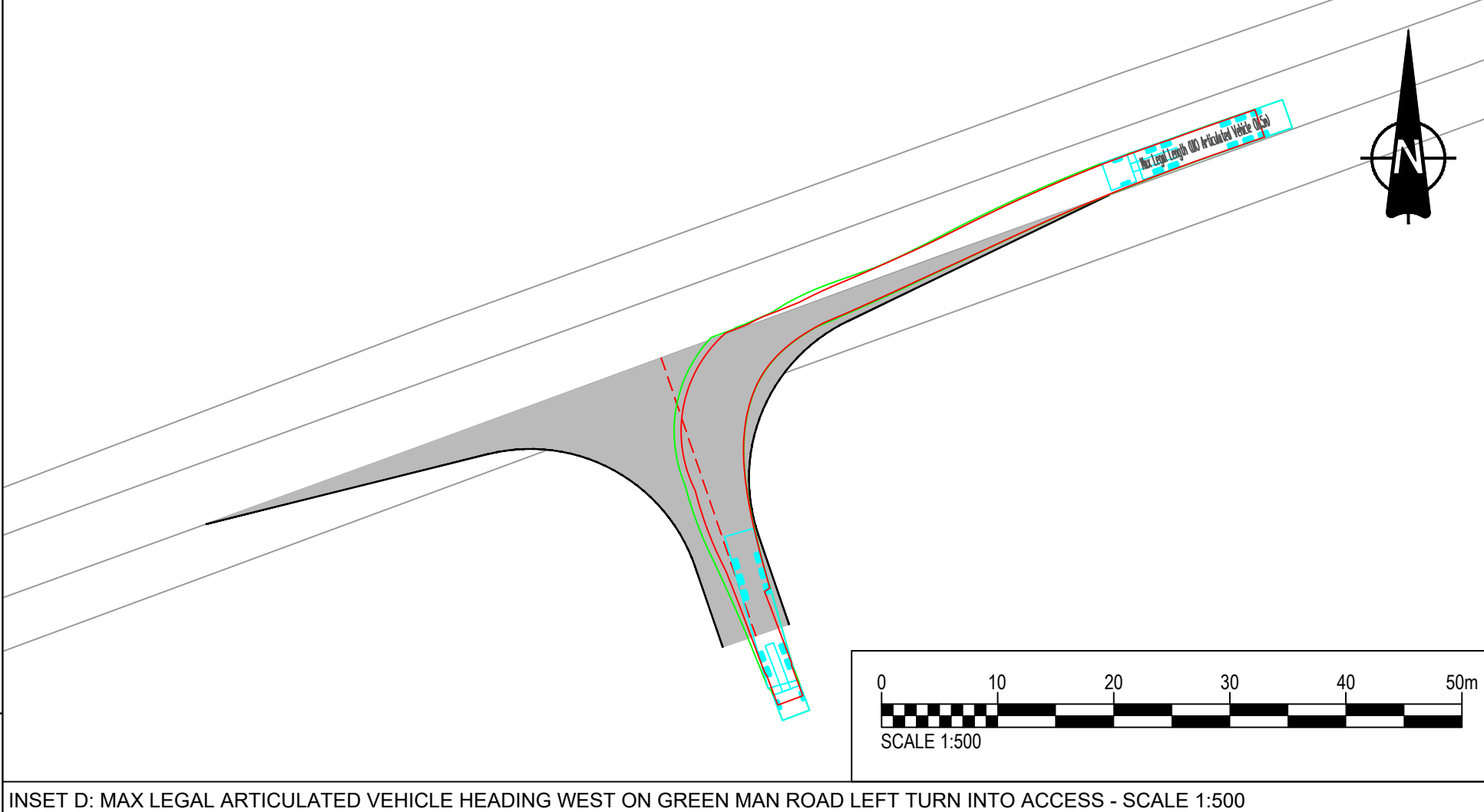
INSET D: MAX LEGAL ARTICULATED VEHICLE HEADING WEST ON GREEN MAN ROAD LEFT TURN INTO ACCESS - SCALE 1:500
